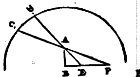
Figura, Solis vmbra oriens, ac se efferens delineans.
